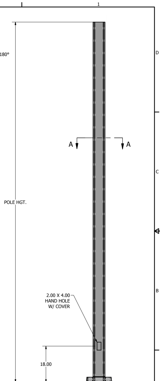
POLE DETAIL
